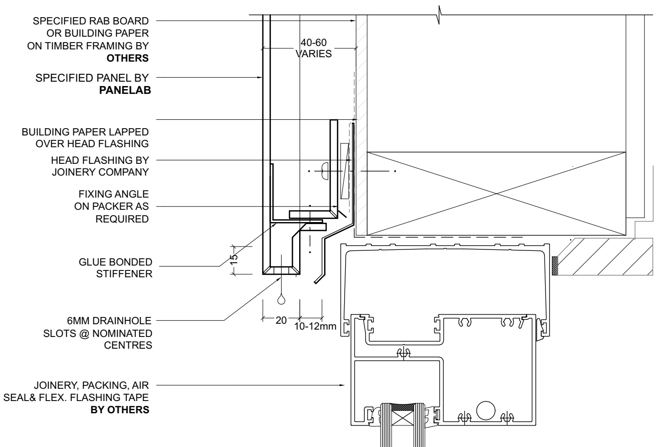
1 TYPICAL COMMERCIAL HEAD DETAIL 1:2 @ A4
