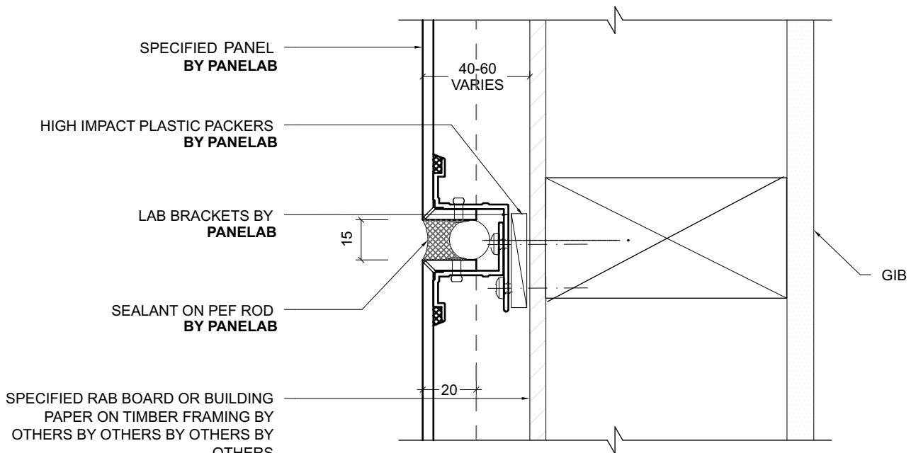
2 TYPICAL HORIZONTAL JOINT (SECTION DETAIL) - 1:2 @ A4
